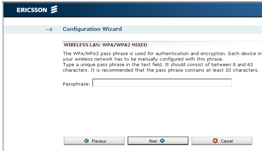
Figure 21 - Wireless LAN: WPA/WPA2 Mixed page
