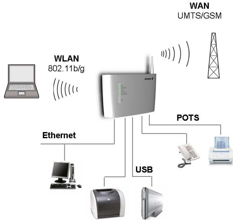
Figure 1 – Ericsson W25 Network Connections
