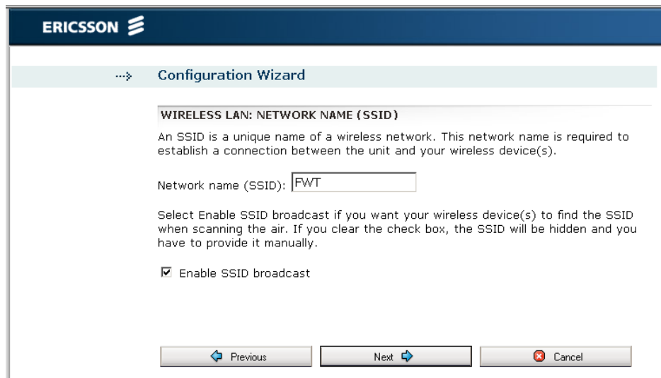
Figure 14 – Wireless LAN: Network Name (SSID) page
