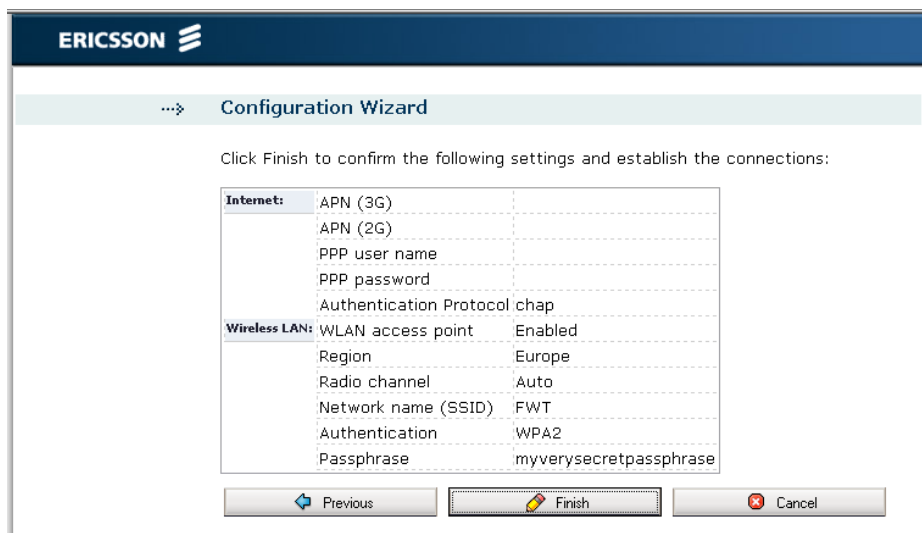
Figure 22 - Configuration Wizard Confirmation page
